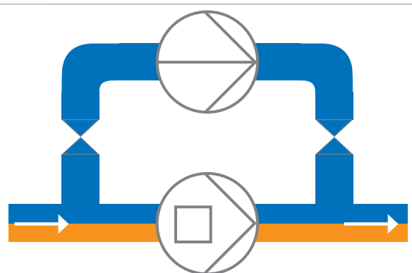
Conveying with displacement pump and CIP-cleaning with centrifugal pump
